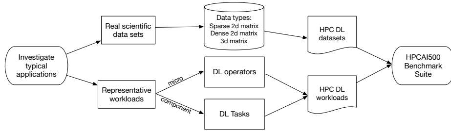
Fig. 1: HPCAI500 Methodology
